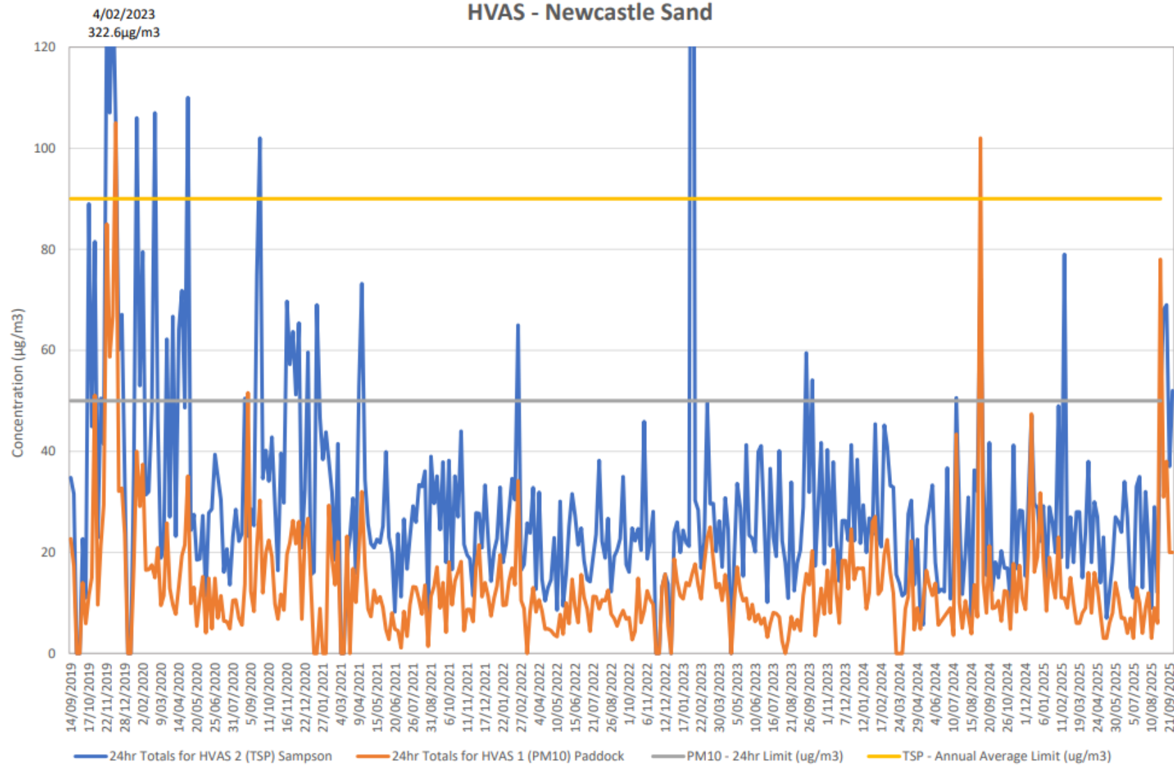
Figure 2 HVAS Long Term Results for TSP and PM10
