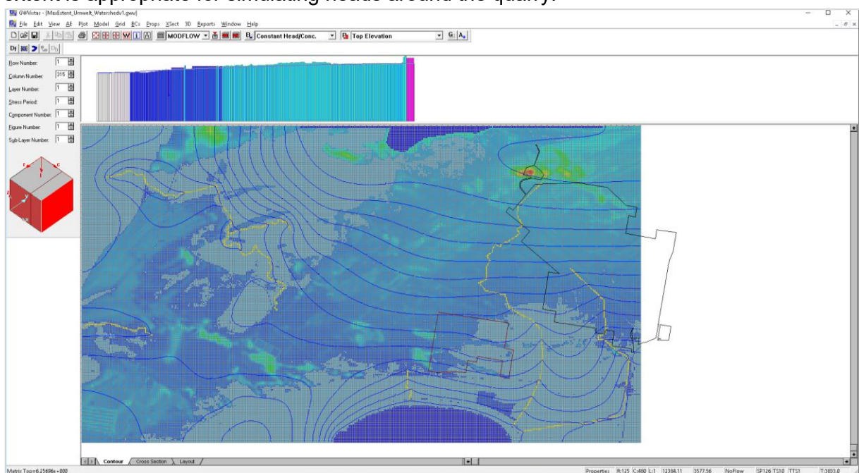
Figure 8: Appendix 3 - Umwelt groundwater model in Groundwater Vistas
