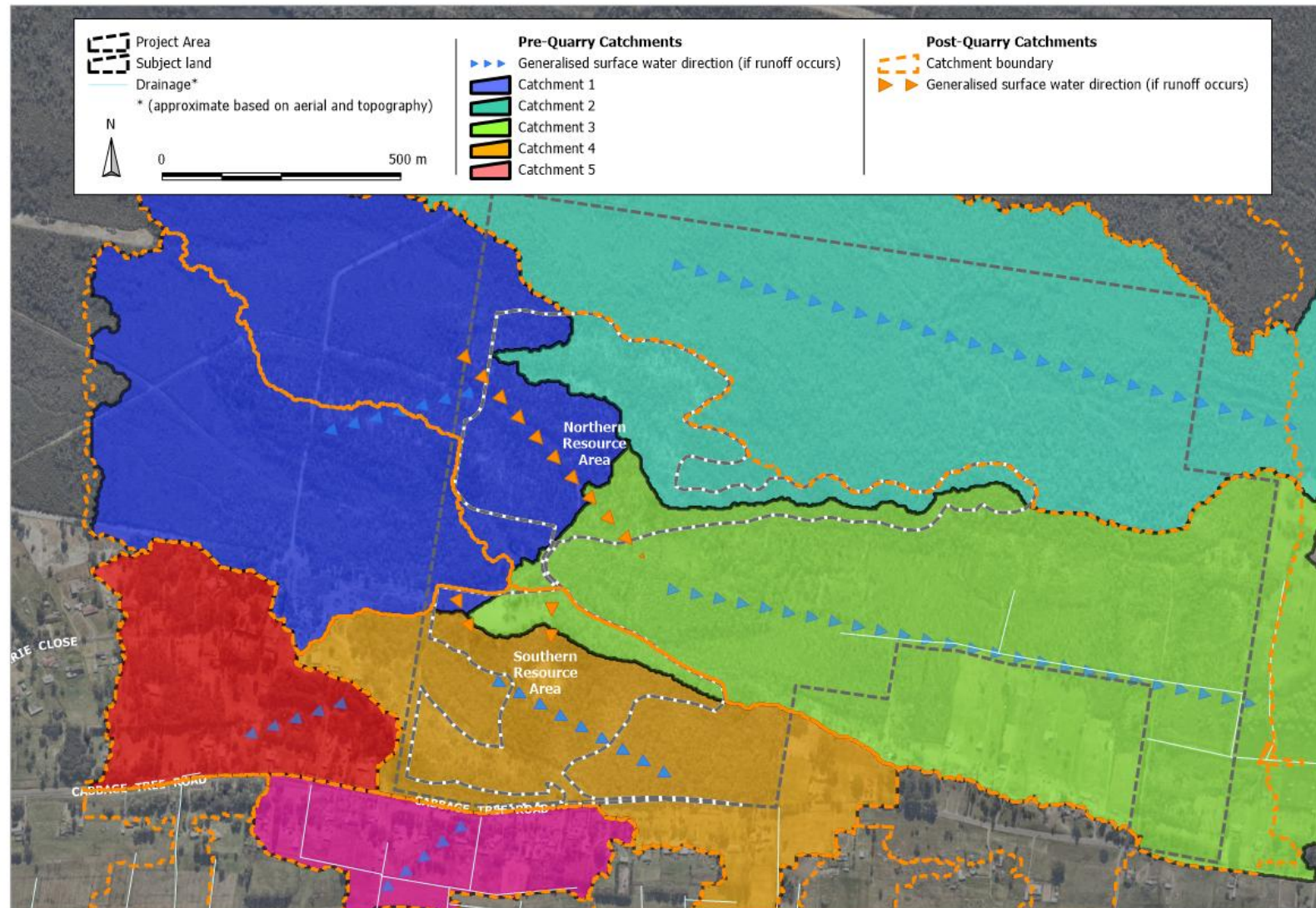
Figure 4: Indicative Pre- and Post-Quarrying Catchment Boundaries and Flow Directions ( if runoff occurred and assuming low areas were filled to overtop )
