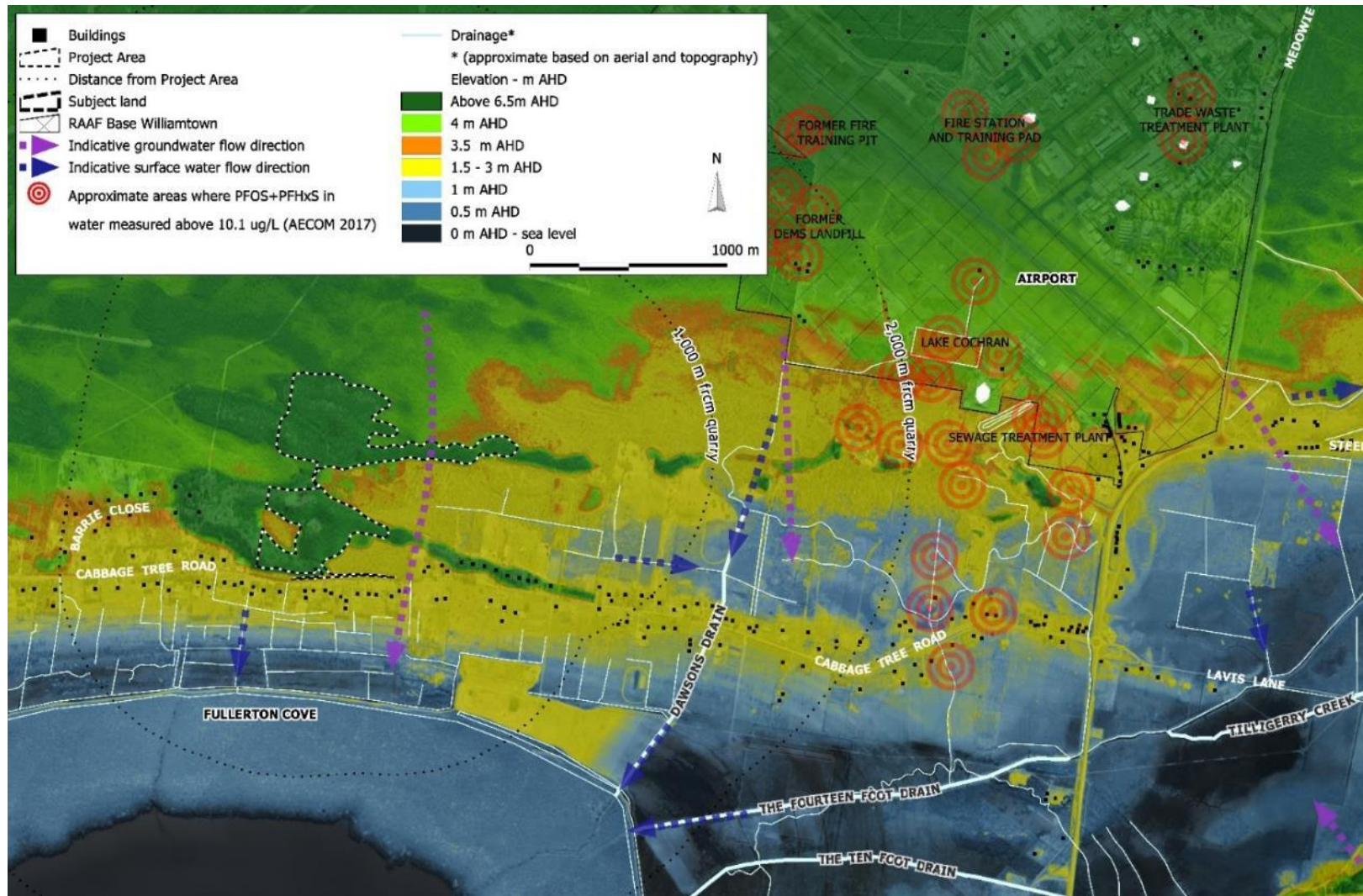
Figure 3: Elevation and Drainage of the Project Area in Relation to Surrounding Lands
